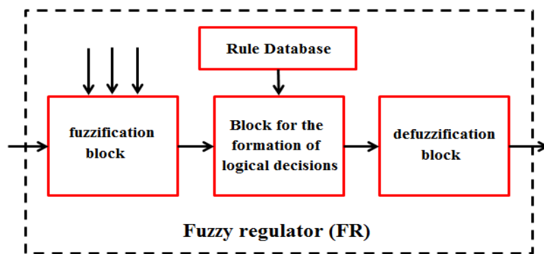
Figure 1. Functional block diagram of fuzzy regulator 1
