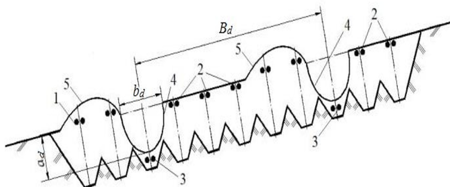
Fig. 1. Scheme of tillage technology with simultaneous sowing of cereals on sloping fields and formation of furrows and ridges against water erosion
