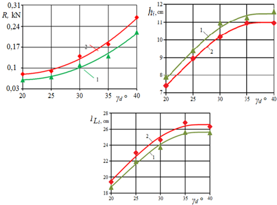
Fig. 5. Mower harvester traction resistance ( R ), mower height ( h_i ), and soil cross-throw masofasi ( L_i ) can be changed depending on installation angle ( \gamma_d ) relative to movement direction of mower harvester
