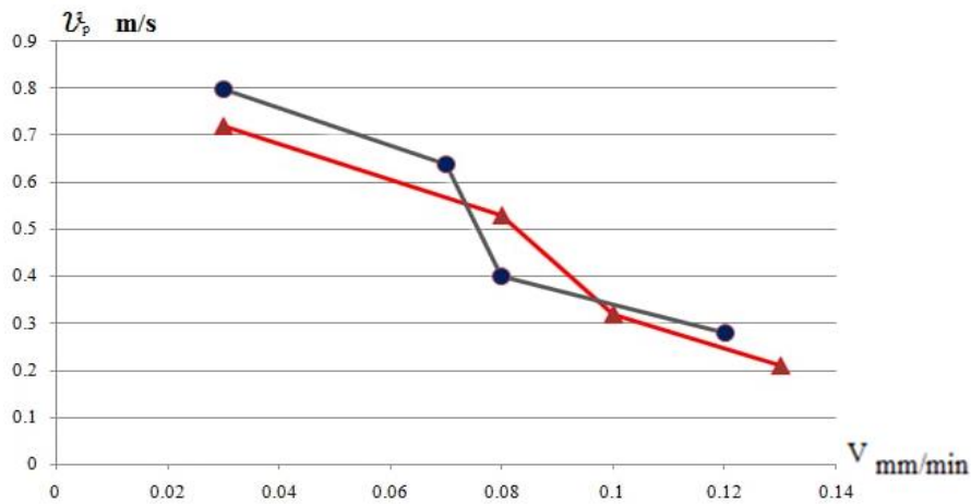
Fig.1. Graph v_p = f(V) of the dependence of the intensity of soil washing on the washing speed
