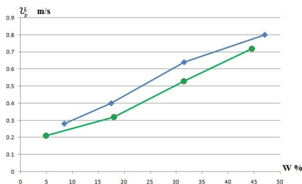
Fig.2. Dependence of flow rate on ground moisture v_p = f(W)
