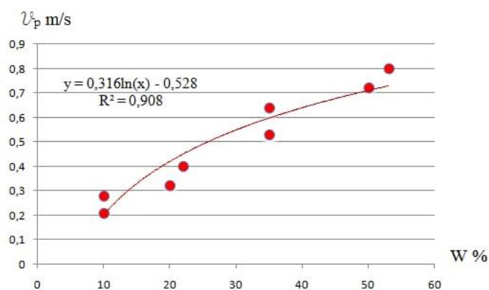
Fig.3. Diagram showing relationships v_p = f(W)
