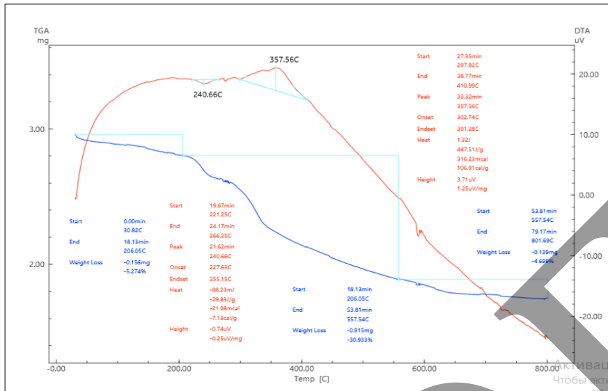
Figure 1. Derivatographic indicators of acrylic-styrene coating
