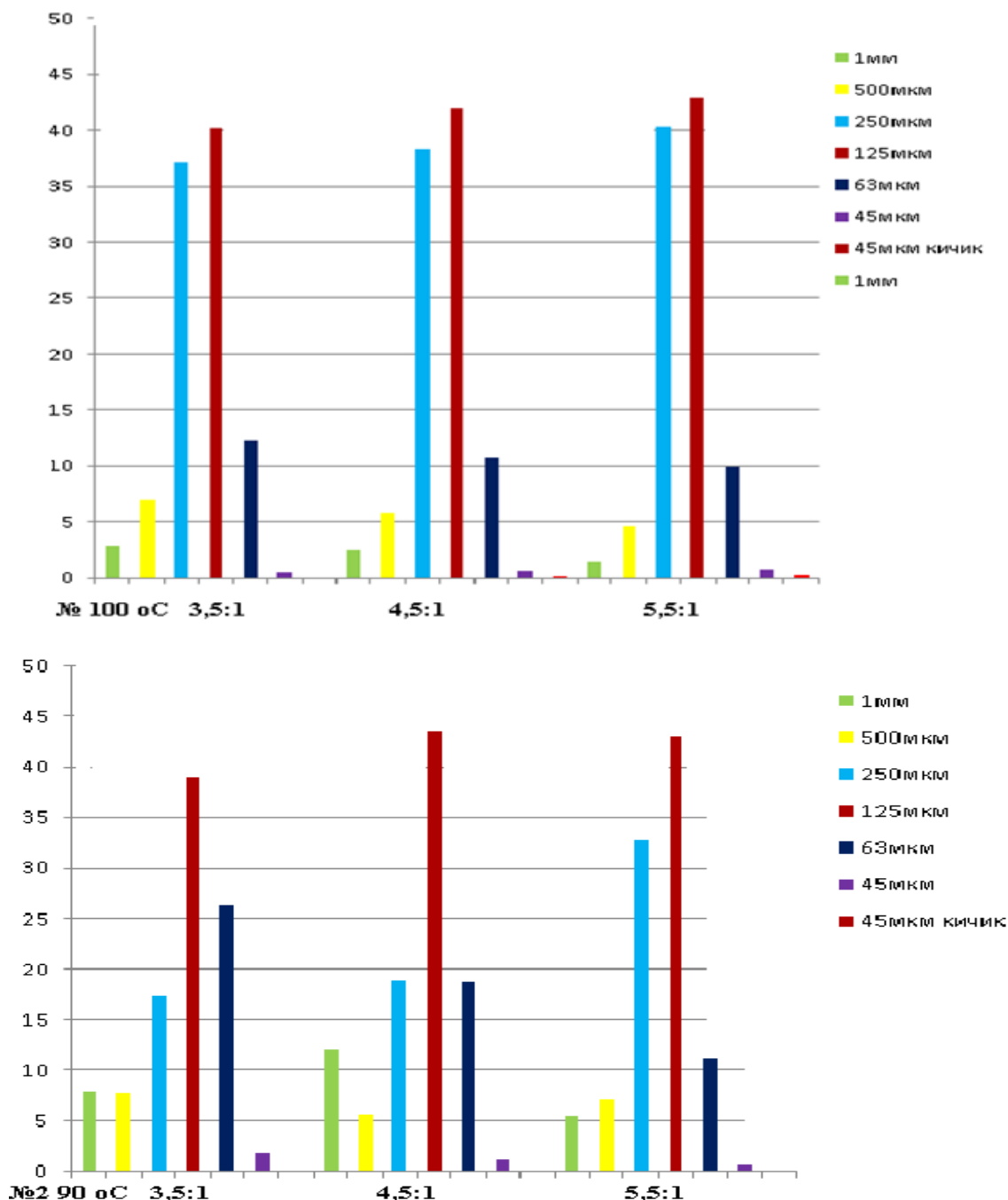
Fig. 1. Granulometric composition of crystalline potassium chloride depending on the process conditions.
