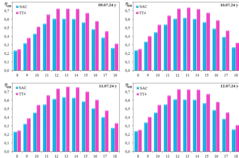
Fig.3. The results of changing the value of energy UWC in the TT4 model.
