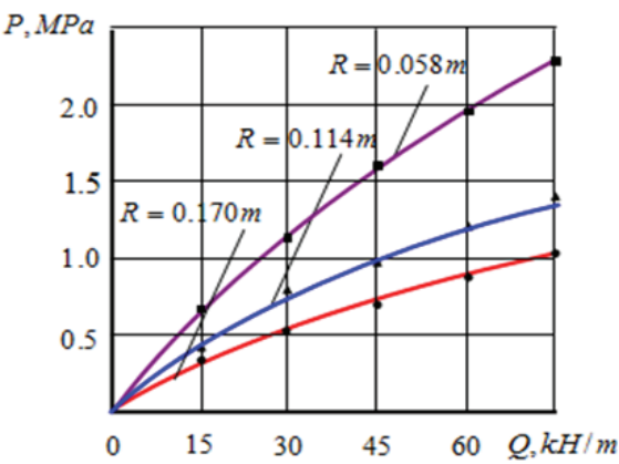
Fig. 1. Dependence of specific pressure from linear pressure.
